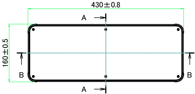
E view
